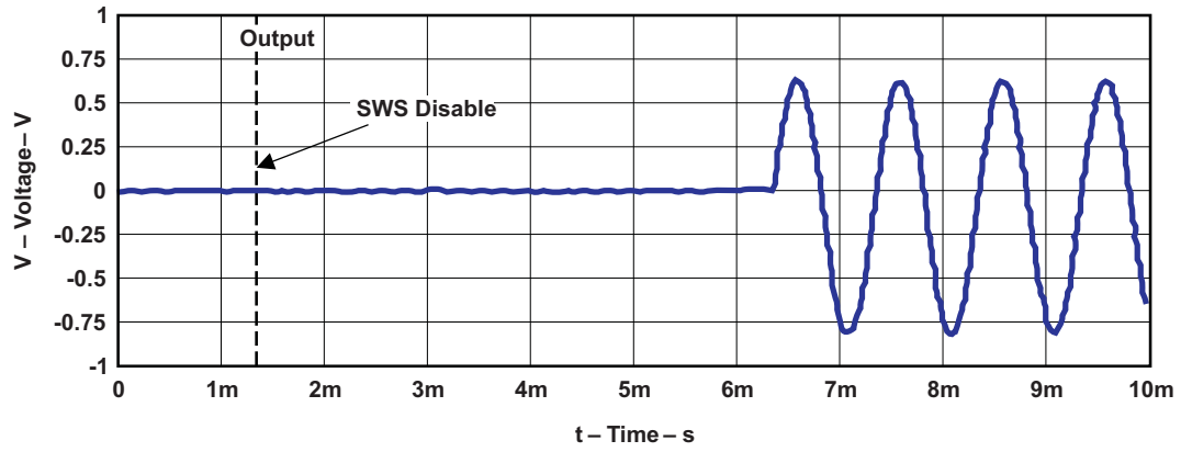
Figure 27. Start-Up Time
