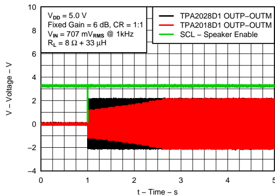
Figure 26. Startup Gain Ramp Comparison
