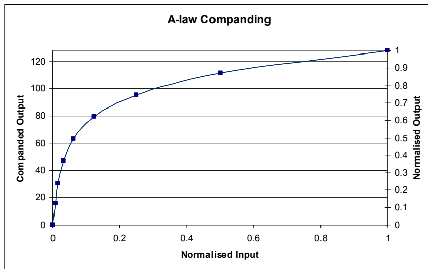
Figure 40 A-Law Comanding
