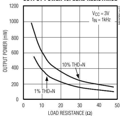
MAX4365 OUTPUT POWER vs. LOAD RESISTANCE
