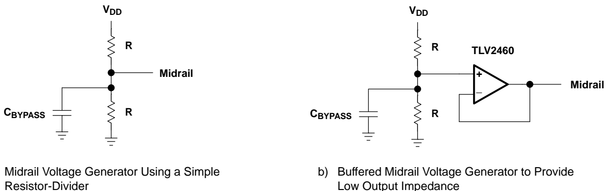
Figure 47. Midrail Voltage Generator
