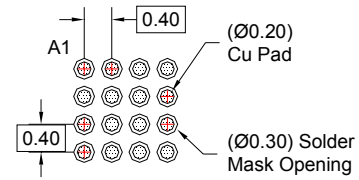
RECOMMENDED LAND PATTERN (NSMD PAD TYPE)
