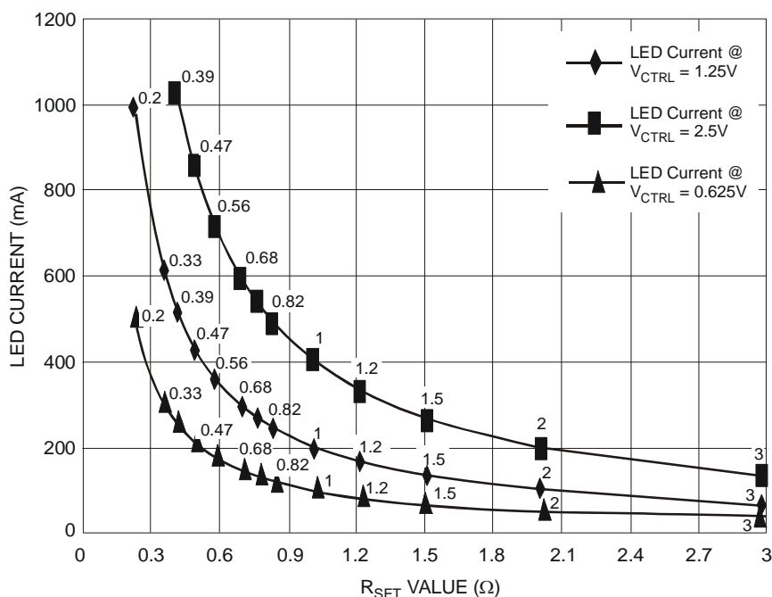
Fig. 19 LED Current Setting vs. R SET and V CTRL
