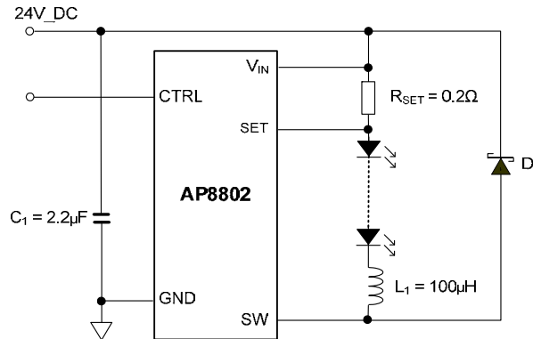
Fig. 14 Typical Application Circuit for I_{LED} = 1A
