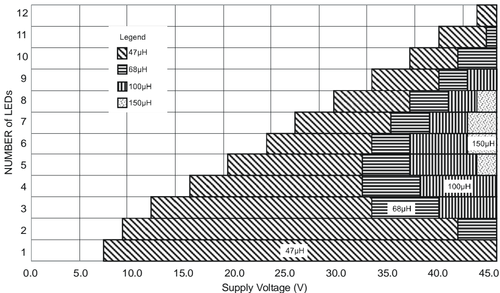
Fig. 16 U-DFN3030-10 Recommended Inductor with 1A LED Current
