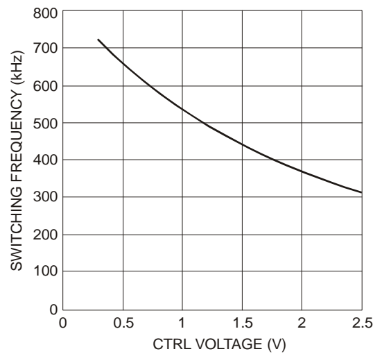
Fig. 7 Switching Frequency vs. V_{CTRL}
