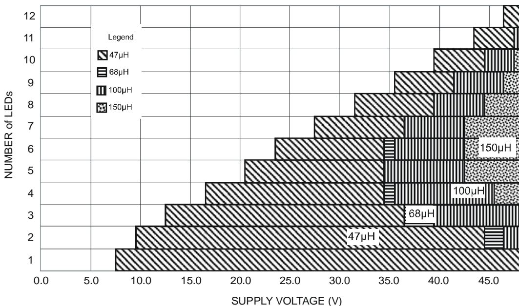
Fig. 17 SO-8EP Recommended Inductor with 1A LED Current
