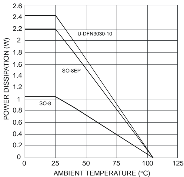
Maximum Power Dissipation Fig. 22 AP8802 Derating Curves
