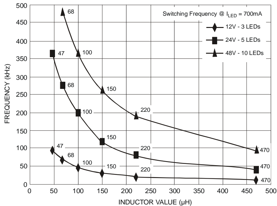
Fig. 15 Switching Frequency vs. Inductor Value
