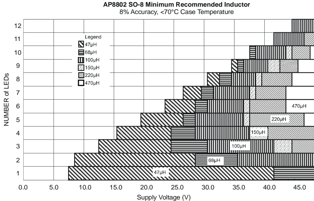
Fig. 18 SO-8 Recommended Inductor with 700mA LED Current
