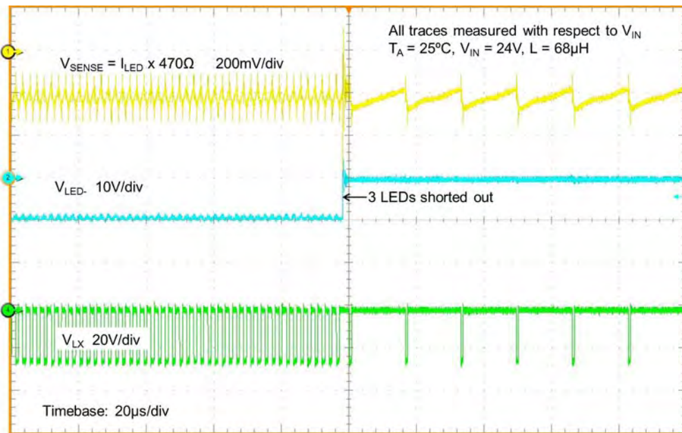
Fig. 24 Switching Characteristics (normal open to short LED chain)
