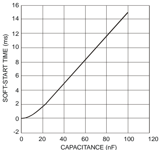
Fig. 21 Soft-Start Time vs. Capacitance from ADJ Pin to Ground
