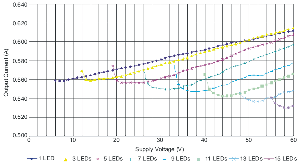
ZXLD1356 Output Current Deviation (Normalized) L = 68μH
