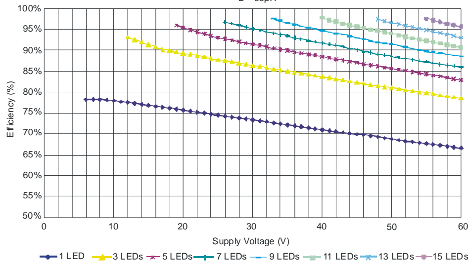
ZXLD1356 Efficiency L = 68μH
