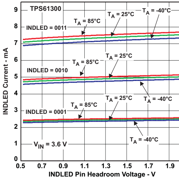
Figure 18. INDLED Current vs. INDLED Pin Headroom Voltage
