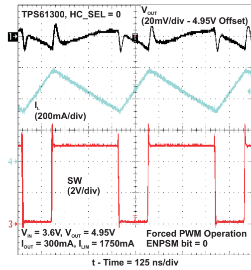
Figure 39. PWM OPERATION
