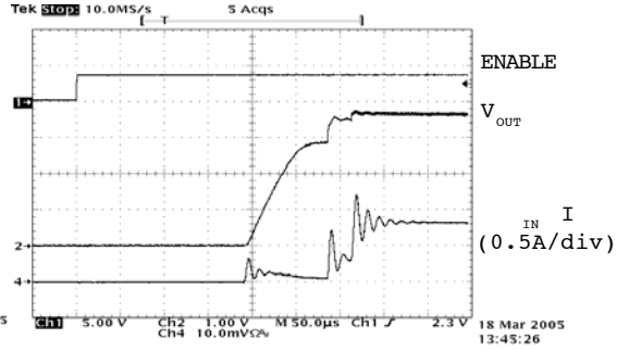
Figure 16. Startup Flash, V_{in}=3.6V , V_{out}=3.5V C_{in}=4.7\mu F , C_{FC}=0.4\mu F , C_{out}=2\mu F
