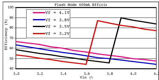
Figure 4. Efficiency vs. Supply Voltage ( C_{IN} = 2.2\mu\text{F} , C_{FC} = 0.47\mu\text{F} , C_{OUT} = 1.0\mu\text{F} )
