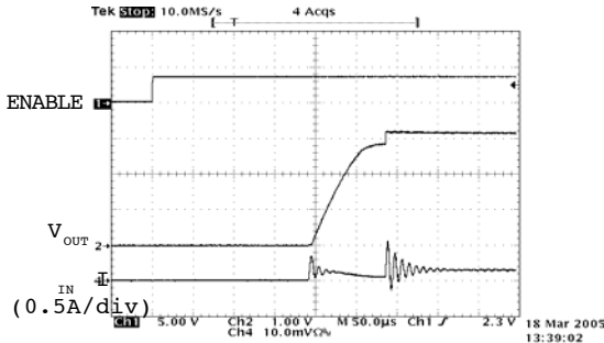
Figure 15. Startup Torch, V_{in}=3.6V , V_{out}=3.1V C_{in}=4.7\mu F , C_{FC}=0.4\mu F , C_{out}=2\mu F
