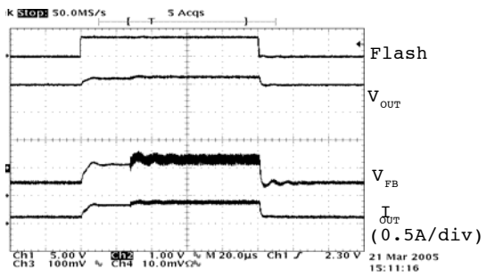
Figure 18. Torch in 1X to Flash 2X Mode, V_{in}=3.6V , C_{in}=4.7\mu F , C_{FC}=0.47\mu F , C_{out}=2.2\mu F
