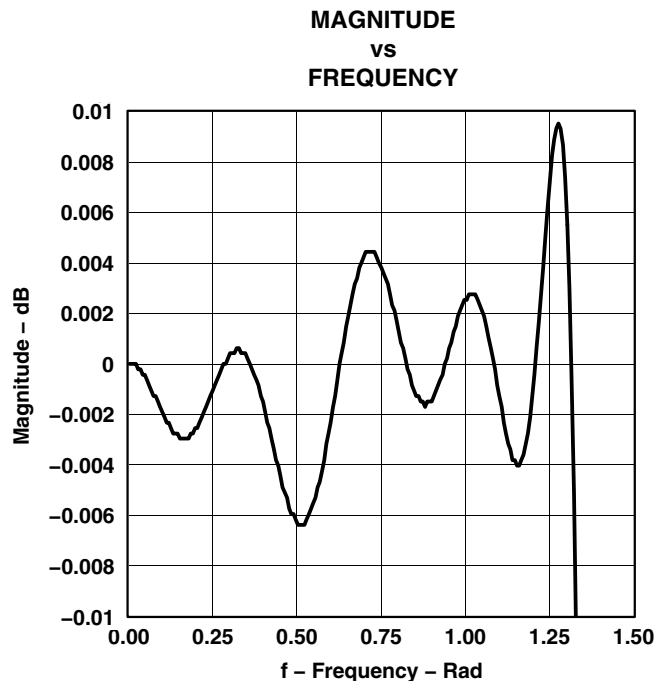
Figure 4-13. IFIR Pass-Band Frequency Response
