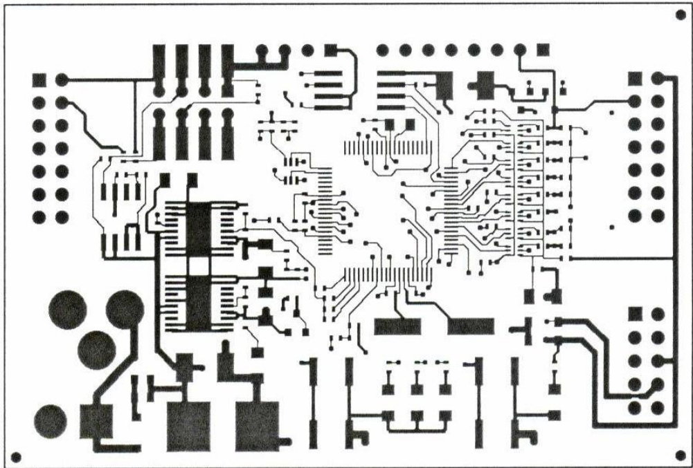
Figure 4.5 - PCB - Top
