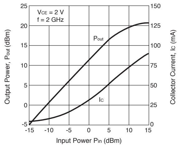
OUTPUT POWER COLLECTOR CURRENT vs. INPUT POWER
