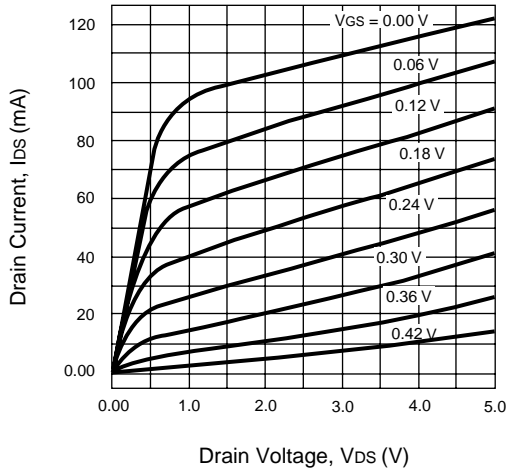
DC PERFORMANCE
