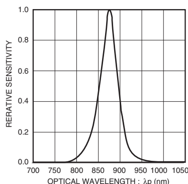
Fig.5 Spectrum data
