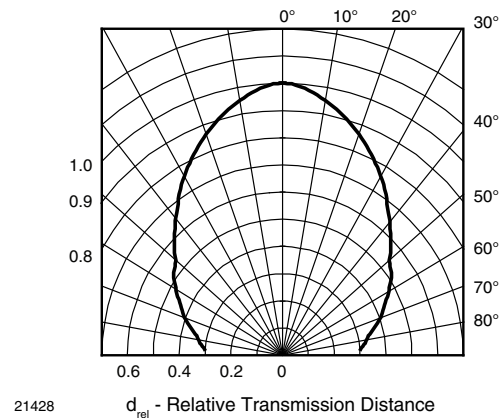
Fig. 13 - Vertical Directivity
