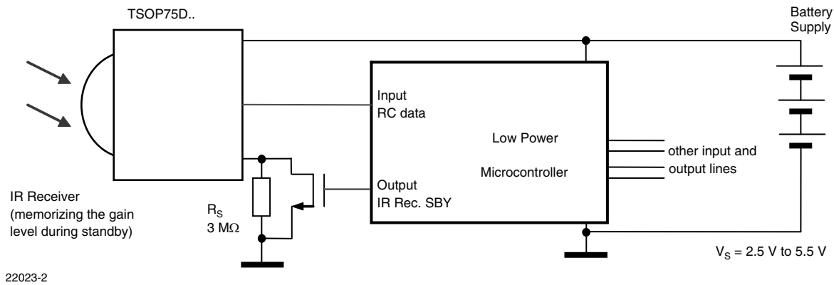
Fig. 17 - Application Circuit for the TSOP75D26 with Intermittent Supply Voltage
