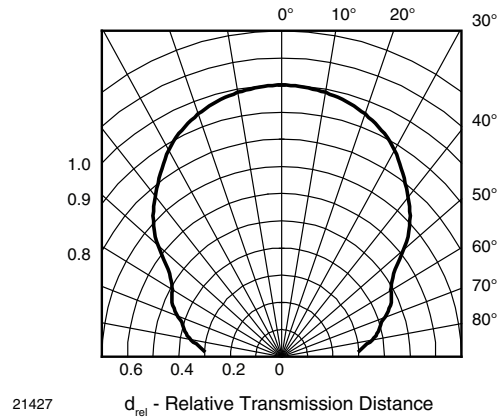
Fig. 12 - Horizontal Directivity
