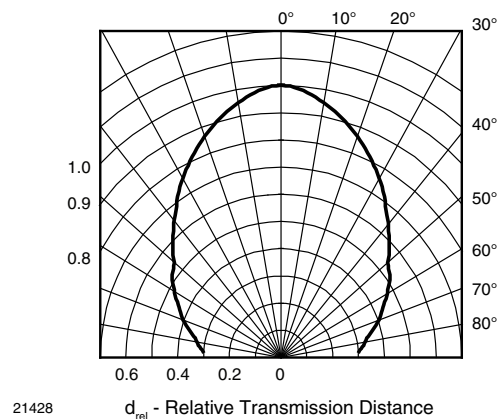
Fig. 4 - Vertical Directivity
