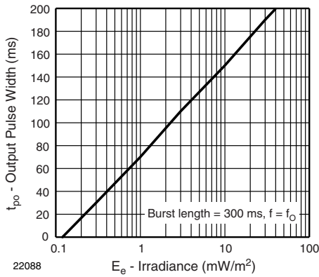
Fig. 9 - Max. Output Pulse Width vs. Irradiance
