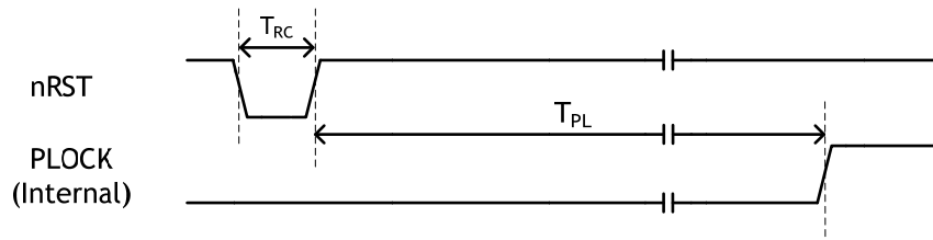
Figure 22 Reset Timing
