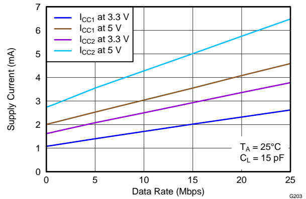
Figure 15. ISO7631FC Supply Current For All Channels vs Data Rate
