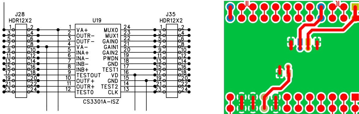
Figure 7. Dual-row Headers with Shorts
