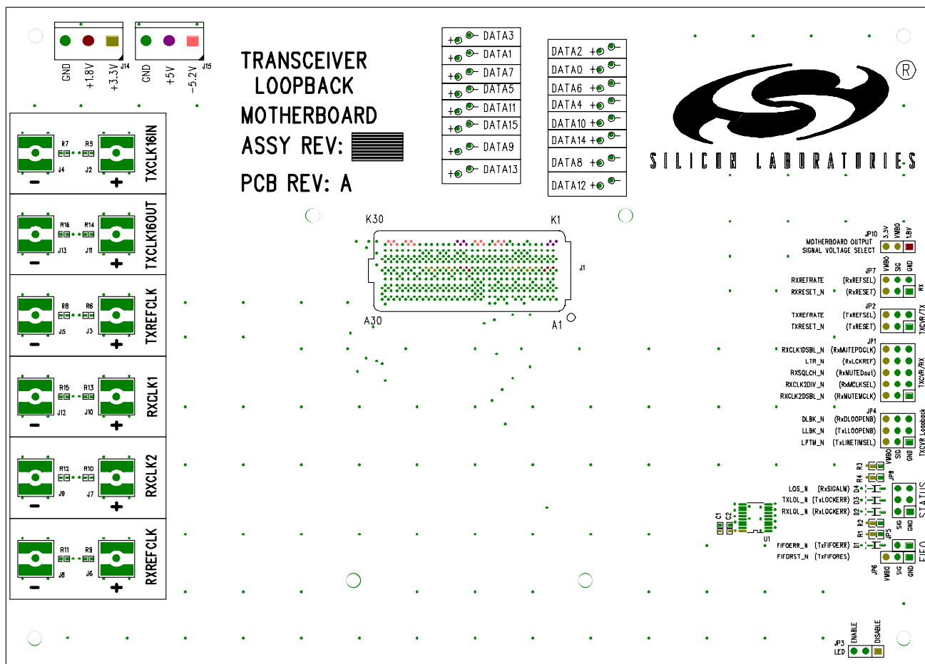
Figure 38. Component Side Assembly (Loopback Motherboard)
