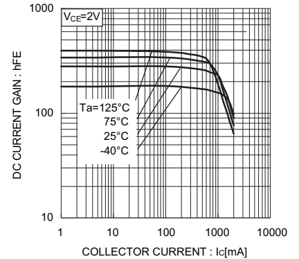
Fig.3 DC Current Gain vs. Collector Current ( II )
