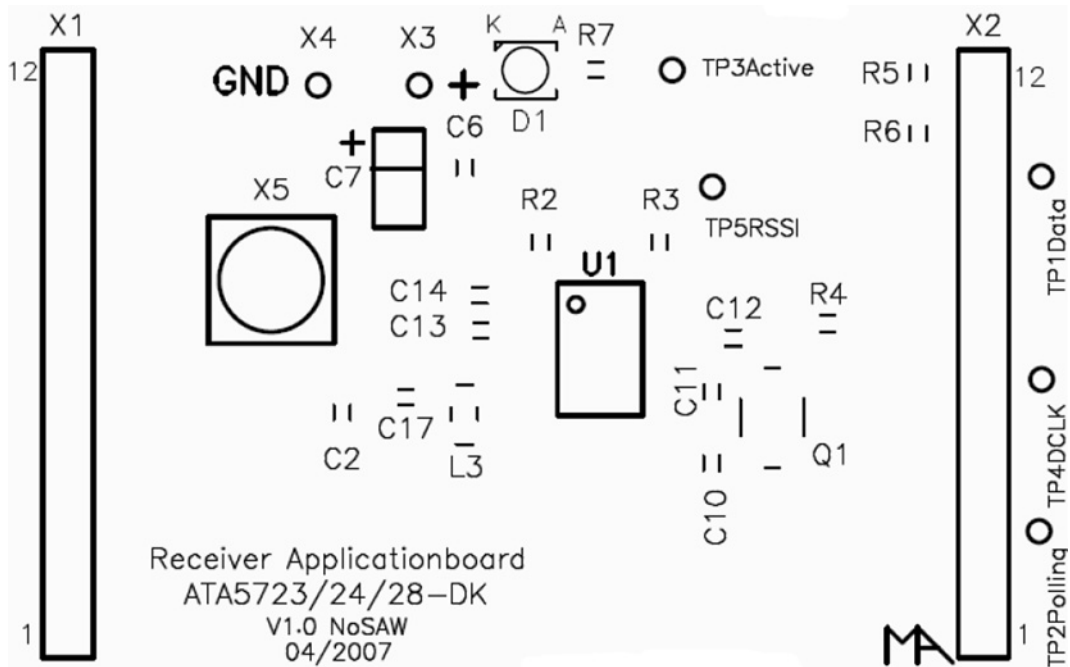
Figure 4-4. Layout of Atmel's Development Board (Designator Layer)
