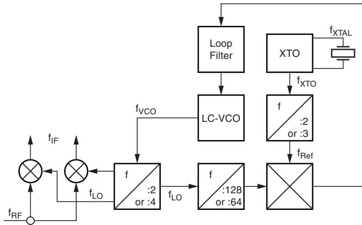
Figure 2-1. System Block Diagram for the Receivers Containing the Internal Frequency Generation and Processing (Synthesizer)
