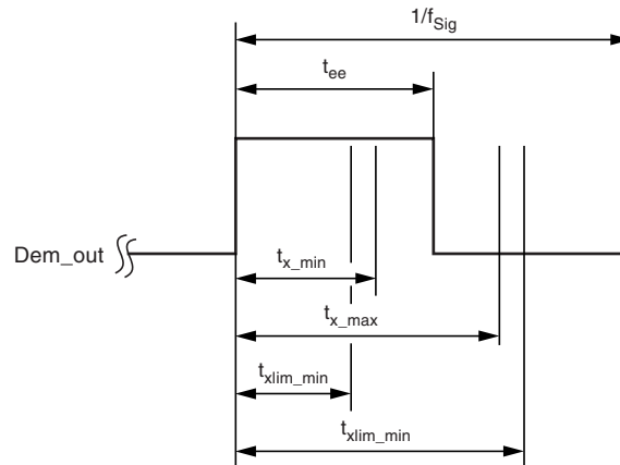
Figure 7-4. The Required Time Limit Ranges for a Successful Bit Check
