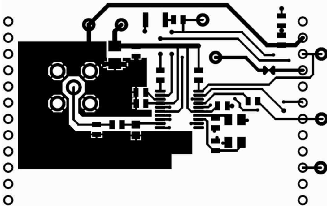
Figure 4-2. Layout of Atmel's Development Board (Top Layer)
