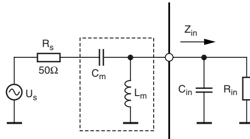
Figure 3-1. LC Matching Network to 50Ω
