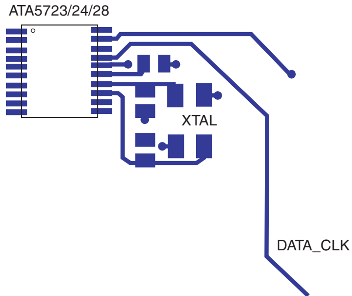
Figure 4-5. An Example of a Bad Wiring of the DATA_CLK Trace
