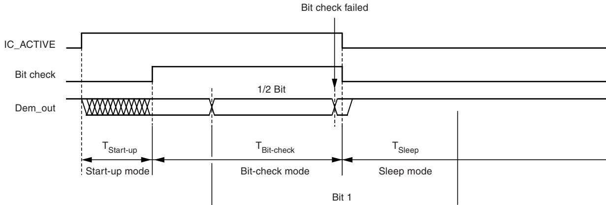
Figure 7-3. Failed Bit Check Processing
