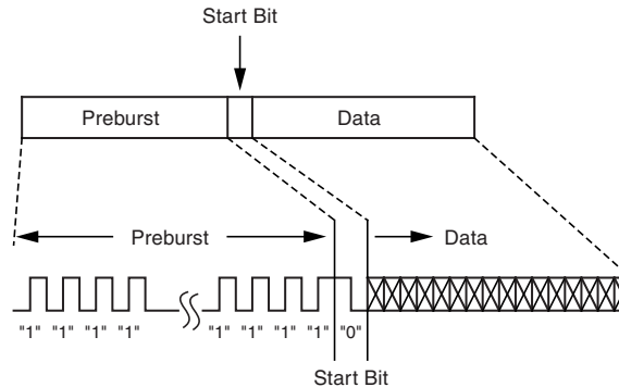
Figure 6-1. The Recommended Protocol (Manchester Coding)
