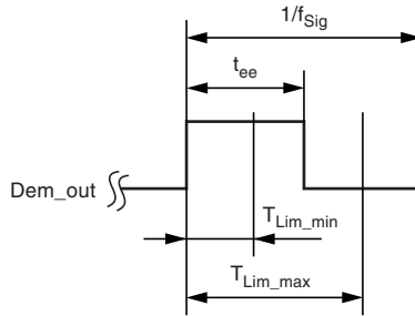
Figure 7-1. Valid Time Window for Bit Check
