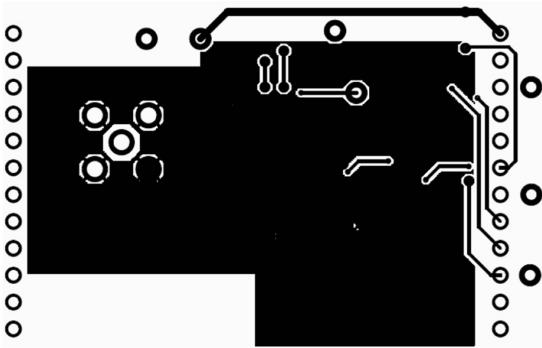
Figure 4-3. Layout of Atmel's Development Board (Bottom Layer)
