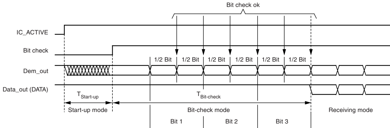
Figure 7-2. Successful Bit Check Processing with Bit Check = 3
