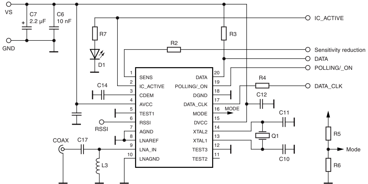
Figure 4-1. Schematic of Atmel's Development Board
