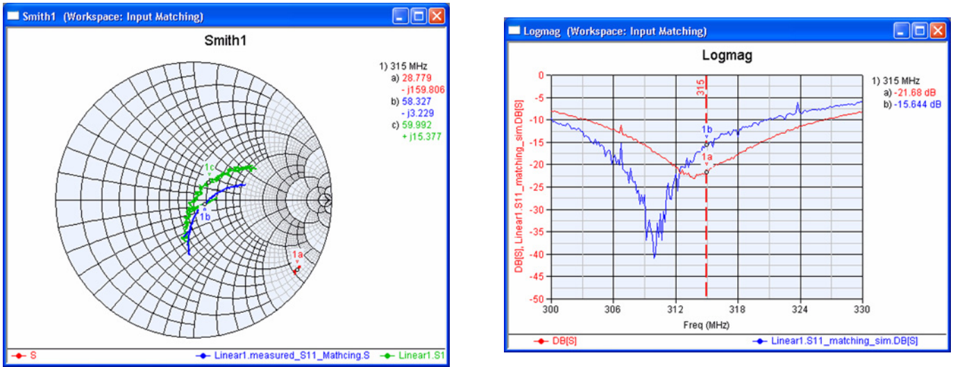
Figure 3-3. Input Impedance of ATA5724 before and after Matching
