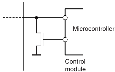
Figure 10-2. Principle Application Circuit with a Switch Transistor Controlling the Serial Data Interface of the Receiver
