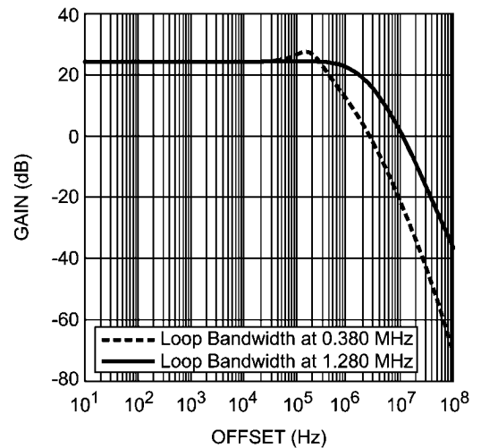
FIGURE 27. PLL Phase Noise Transfer Function: ADC CLK = 50 MHz
