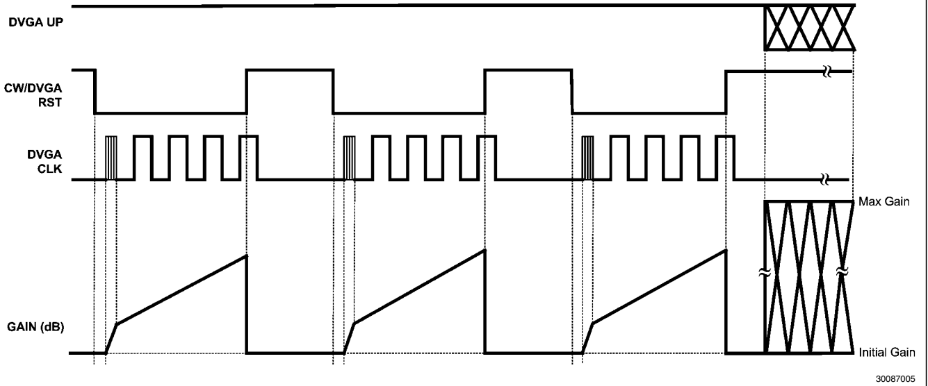
FIGURE 19. Periodic TGC Ramp: Example 2 (Half Step Disable bit = 1)
