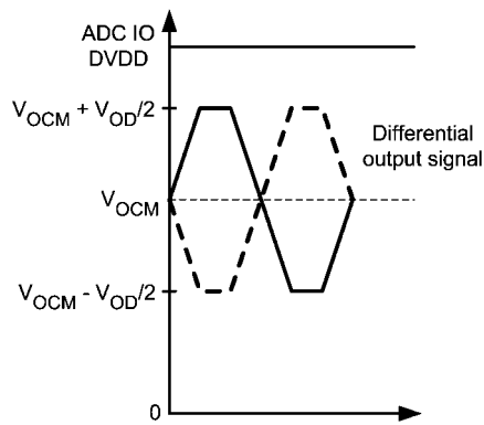
FIGURE 6. B-Mode ADC Data Output Level Definitions
