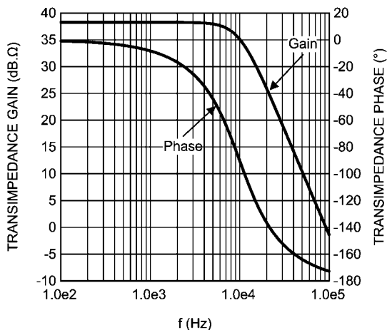
FIGURE 36. CW Doppler LFP Gain/Phase Characteristics
