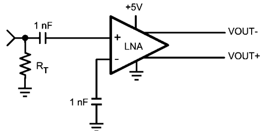
FIGURE 13. Standard Input Termination
