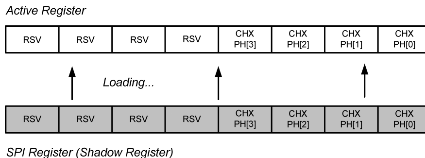
Figure 41. CW Doppler Shadow Register Representation
