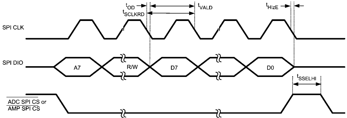
FIGURE 9. SPI™ Read Timing
