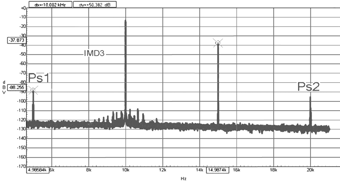
CW Doppler IMD3, Unequal Tones See Electrical Characteristics ( Note 13 ), 10kHz & 15kHz Offset, 25 dB Separation
