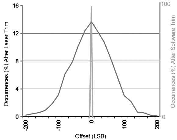
FIGURE 15. Offset Distribution Histogram including Soft-Trim Improvement
