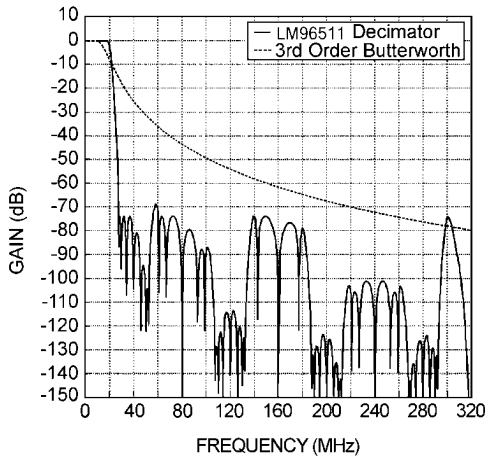
FIGURE 28. Digital Filter Transfer Function
