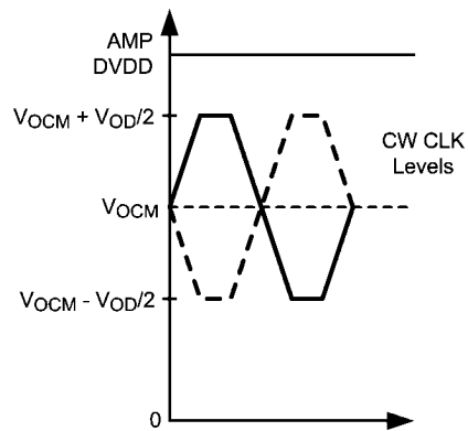
FIGURE 7. CW CLK Level Definitions
