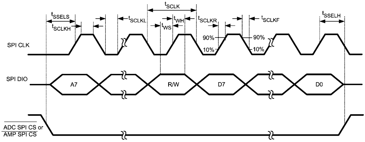
FIGURE 8. SPI™ Write Timing
