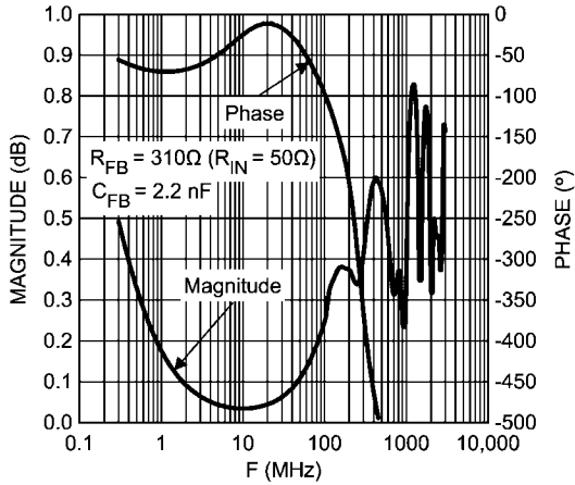
LNA S11 vs. Frequency
