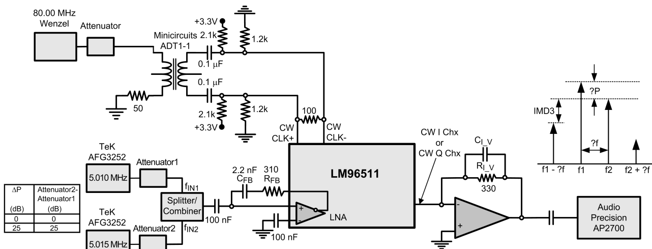
FIGURE 3. Intermodulation Distortion Measurement with Unequal Tones
