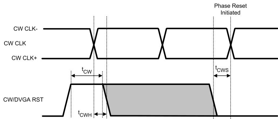
FIGURE 10. CW/DVGA RST Timing (CW Doppler Mode)
