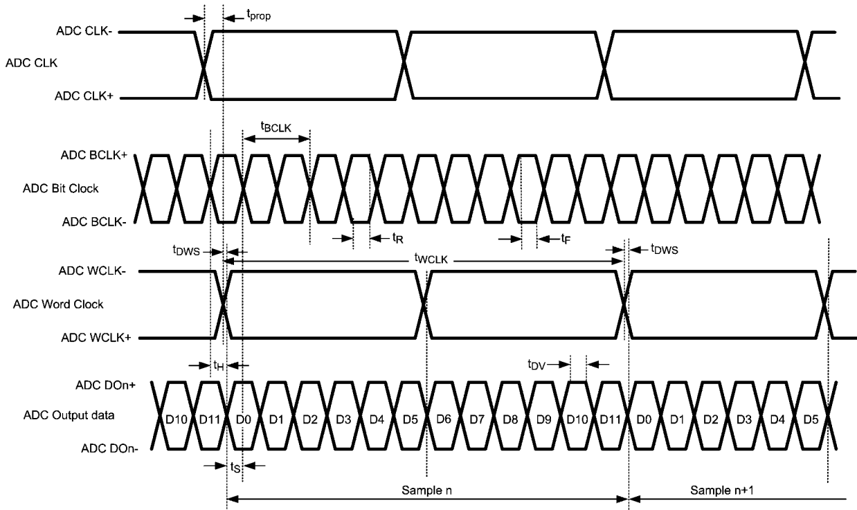
FIGURE 5. B-Mode ADC Data Output Timing
