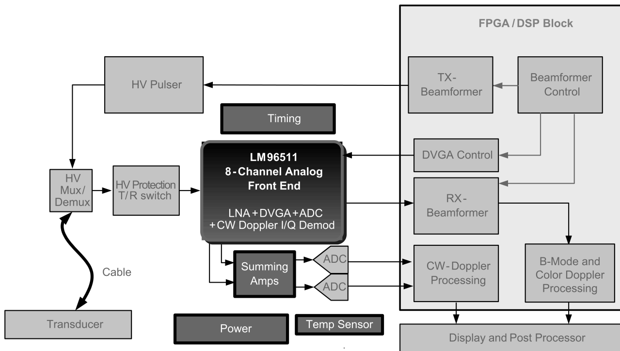
FIGURE 11. Ultra-Sound System Block Diagram
