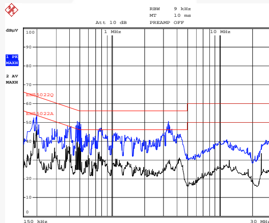
Figure 17. L: 115 / 60Hz
