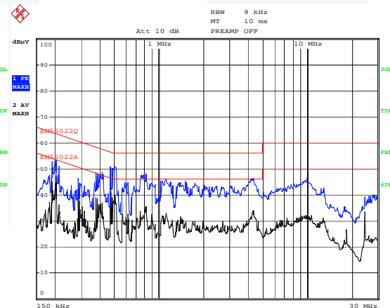
Figure 18. N: 115 / 60Hz
