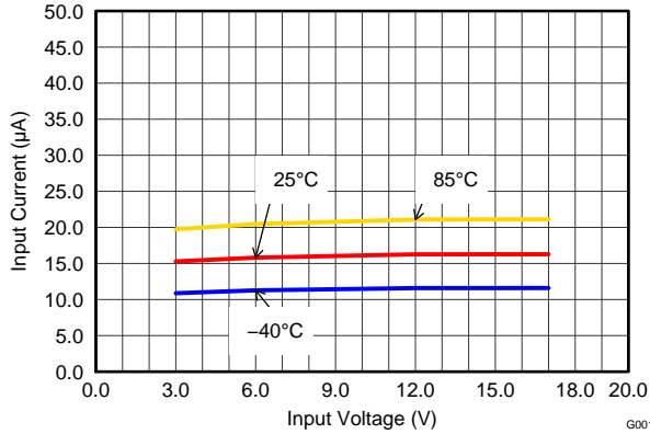
Figure 17. Quiescent Current
