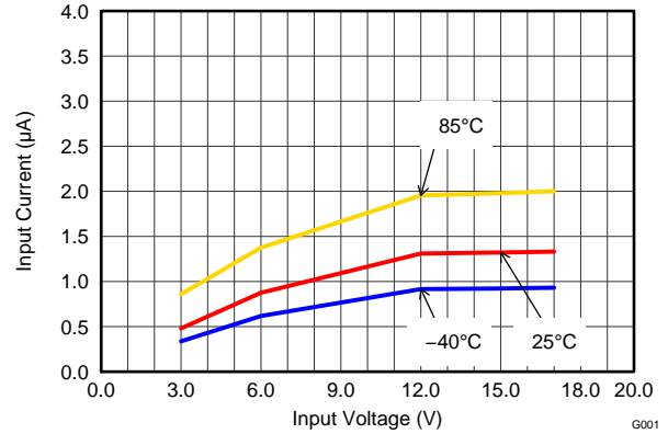
Figure 18. Shutdown Current
