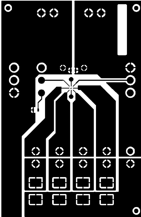
Figure 4. LP5524 Evaluation Board Layer 1 (Top). 30035310
