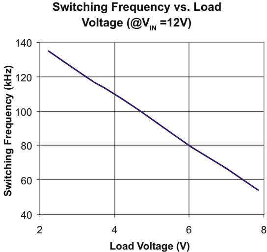
Fig. 10. Switching Frequency vs. Load Voltage Plot
