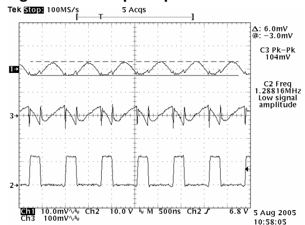
Figure 8. Output Ripple
