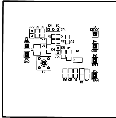
FIGURE 8. Silk Screen—Si9181
