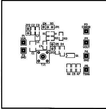
FIGURE 12. Silk Screen—Si9182
