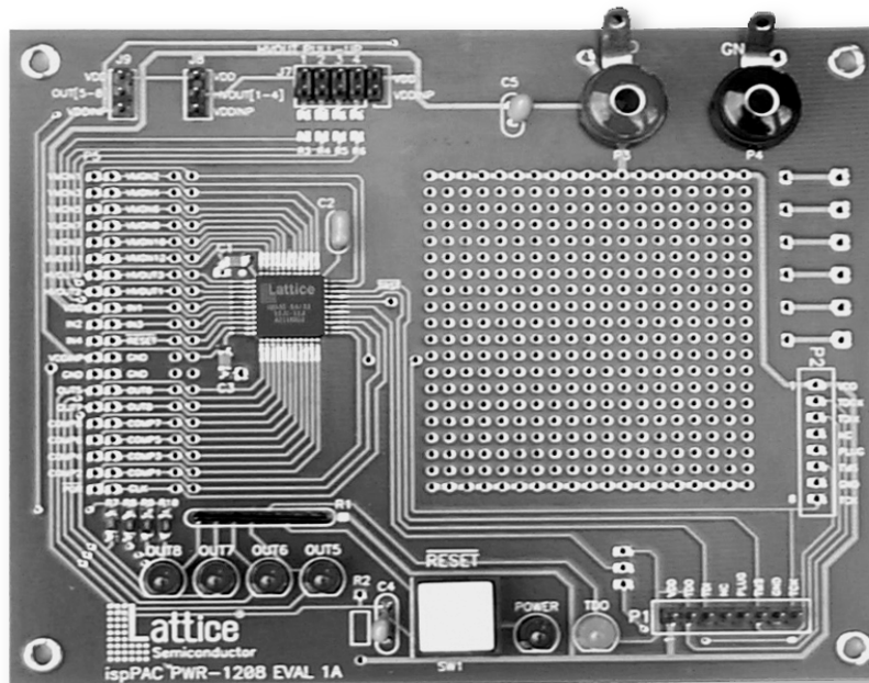
Figure 1. PAC-POWR1208P1-EV Evaluation Board
