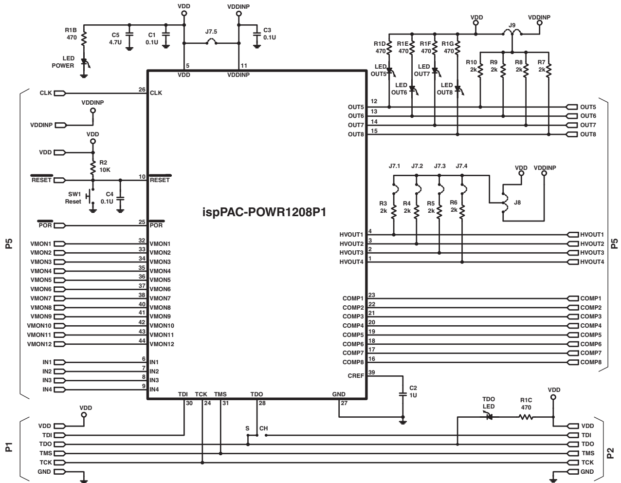
Figure 2. Schematic
