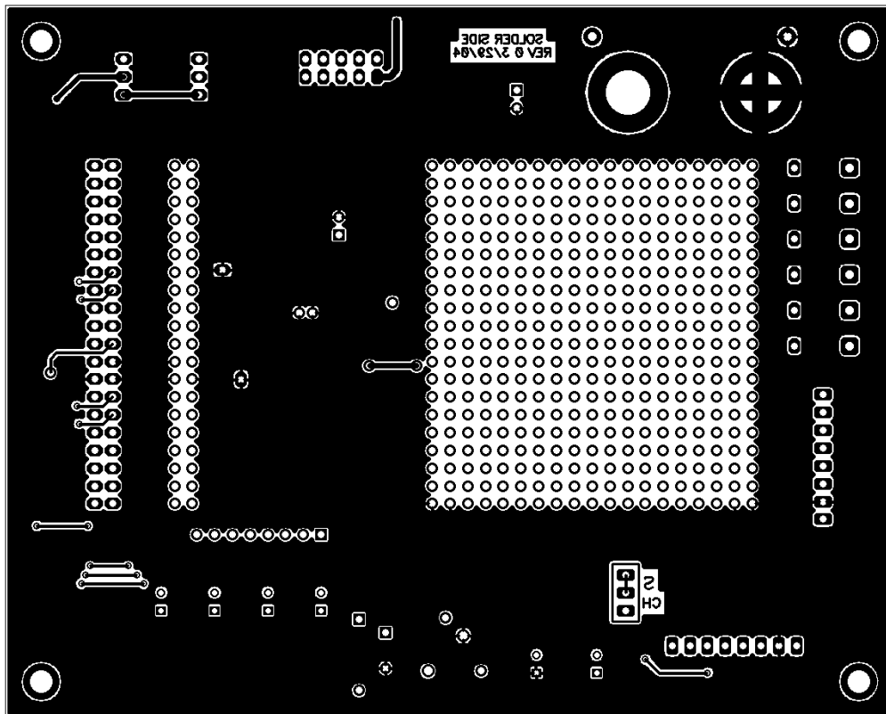
Figure 6. Bottom-side Foil
