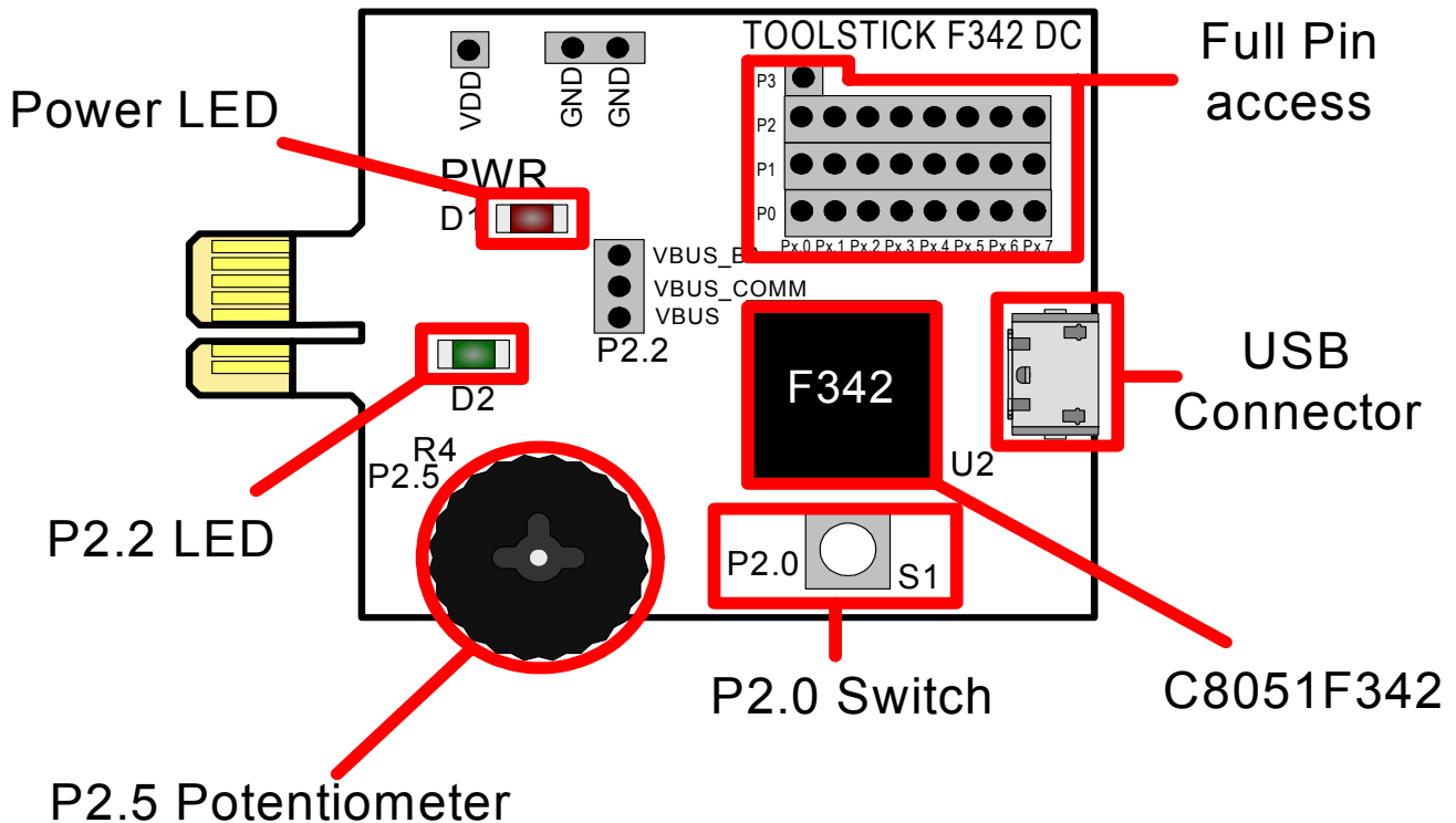
Figure 3. ToolStick C8051F342 Daughter Card
