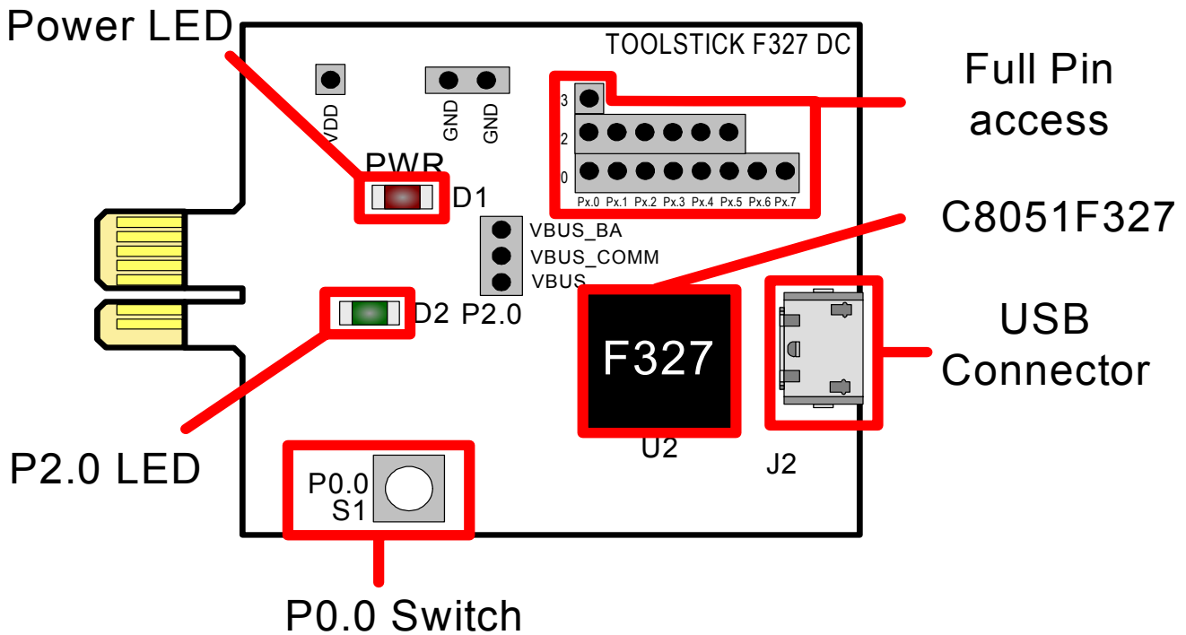
Figure 3. ToolStick C8051F327 Daughter Card
