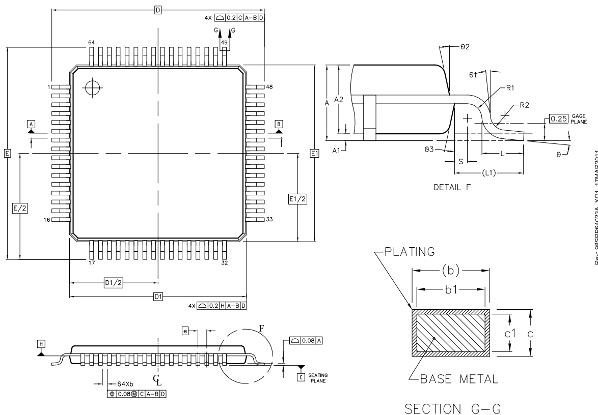
Figure 4.2. TQFP64
