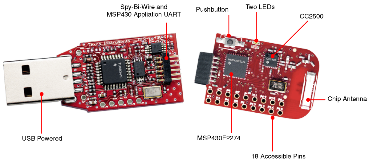
Figure 1. eZ430-RF2500
