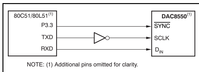
Figure 50. DAC8550 to 80C51/80L51 Interface
