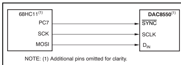
Figure 52. DAC8550 to 68HC11 Interface
