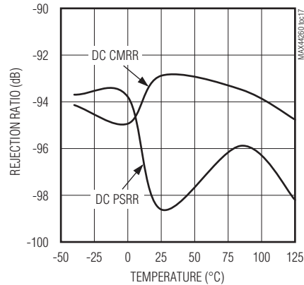
DC CMRR AND PSRR vs. TEMPERATURE
