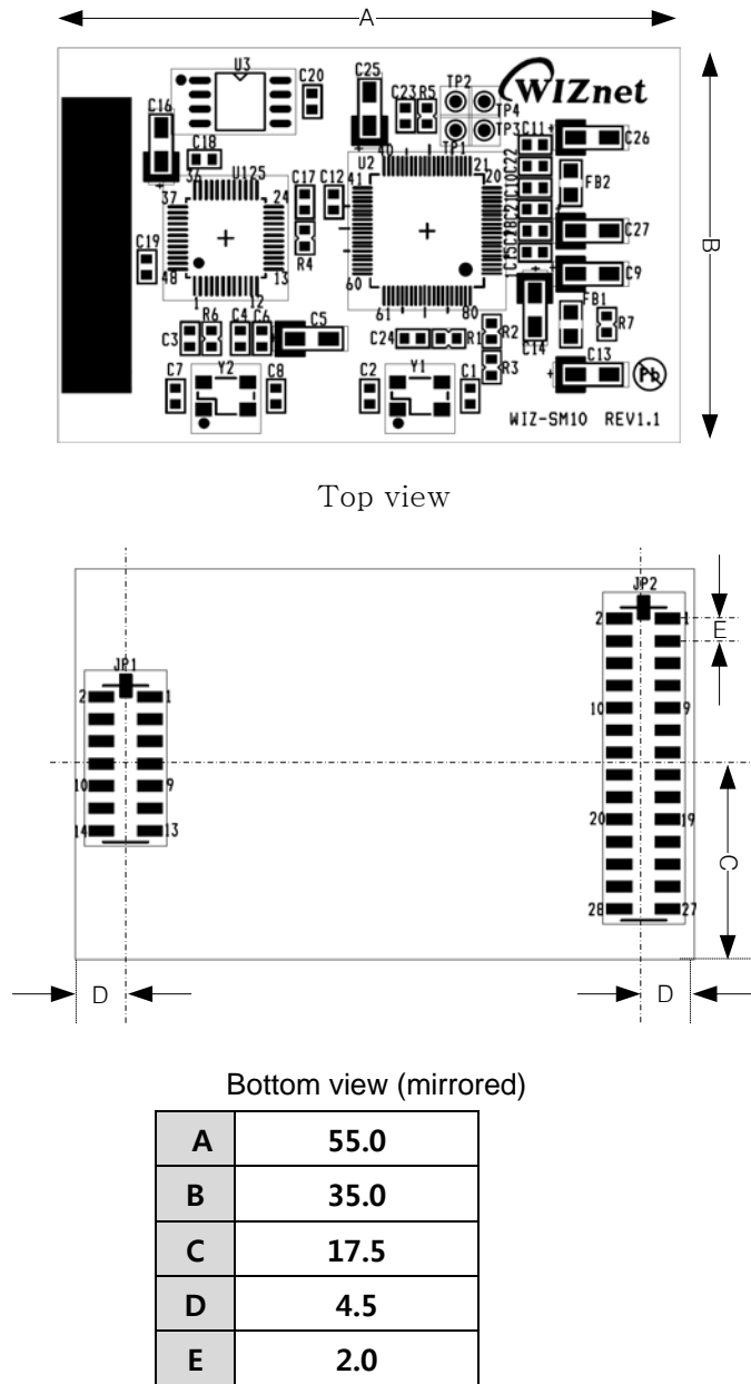
Figure 2. WIZ-SM10 Dimensions (unit: mm)
