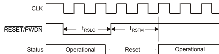
Figure 42. DAC \overline{\text{RESET/PWDN}}
