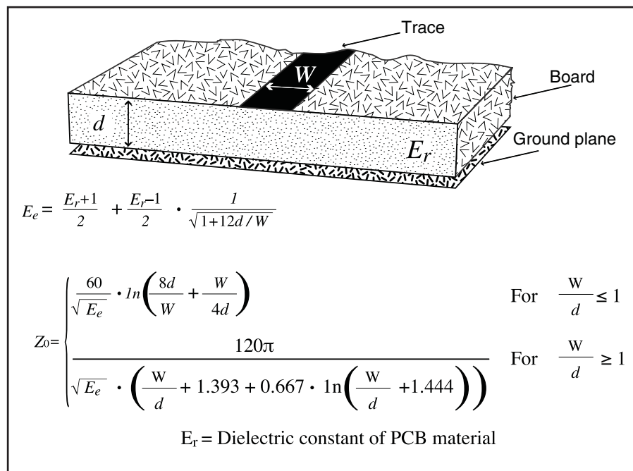
Figure 12: Microstrip Formulas
