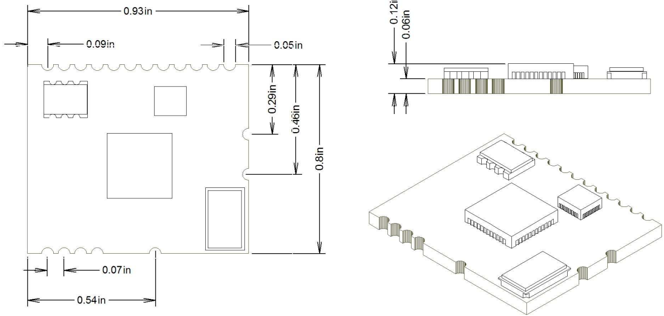
Figure 7: Module Mechanical Drawings
