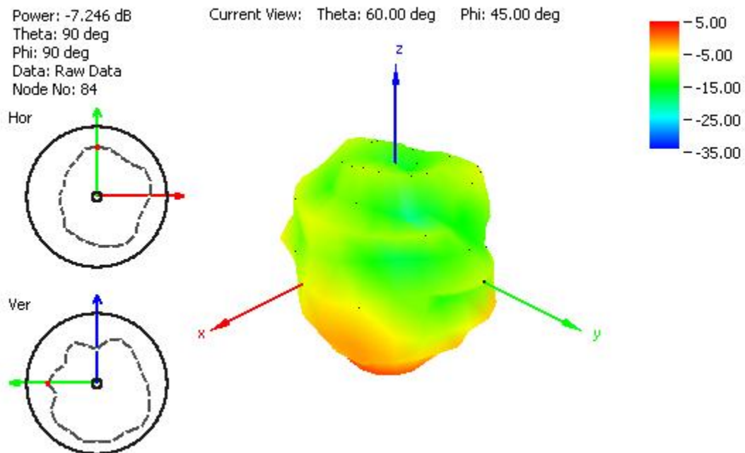
Figure 17. Radiation pattern at 915 MHz, Figure 1 as reference (dB),
