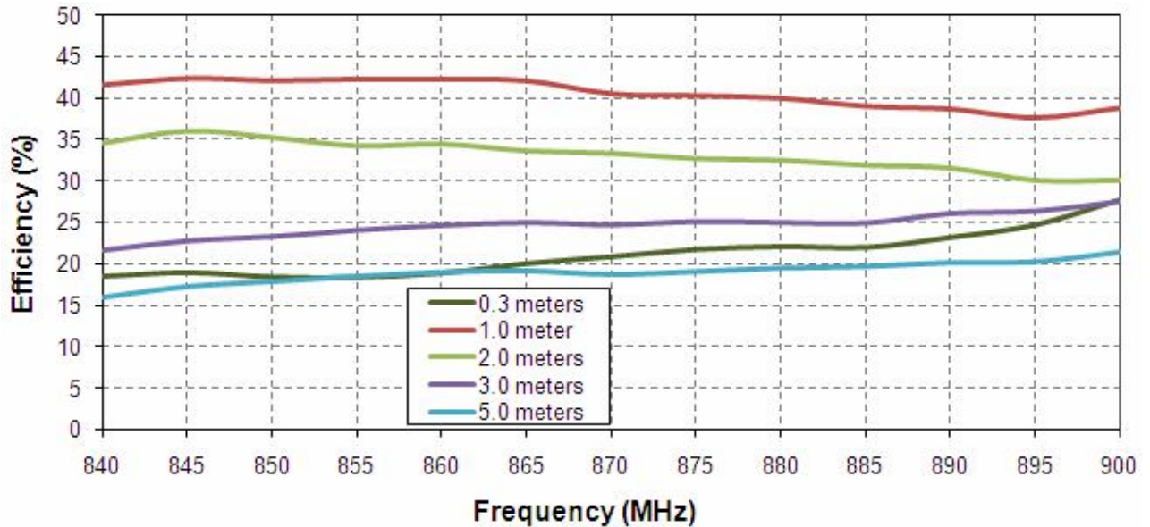
Figure 7. Efficiency of the 868MHz Hercules ISM antenna on 60x60 cm metal plate.
