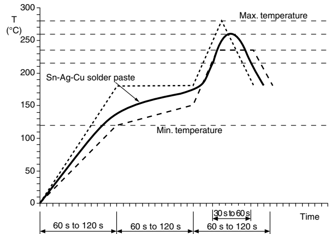
Fig. 10 - Soldering IR Reflow with SnAgCu Solder
